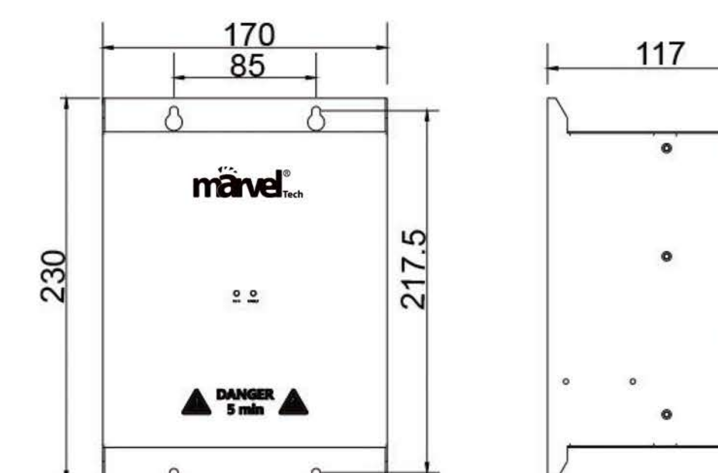
Installation dimension
